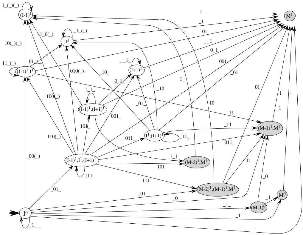
Figure 6 The universal deterministic Levenshtein automaton A^\vee(1) . See Example 4 for notation.
