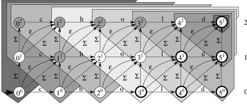
Figure 4 Nondeterministic automaton A(\text{chold}, 2) for testing Levenshtein distance with bound k = 2 for pattern “chold”. Triangular areas are highlighted. Dark states are active after reading symbols h and c .
