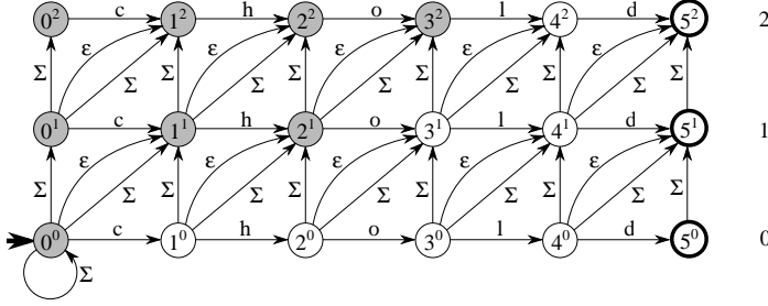
Figure 3 Nondeterministic automaton A_{AST}(\text{chold}, 2) for approximate search with pattern “chold” and distance bound k = 2 . Active states after reading symbols t and h are highlighted.
