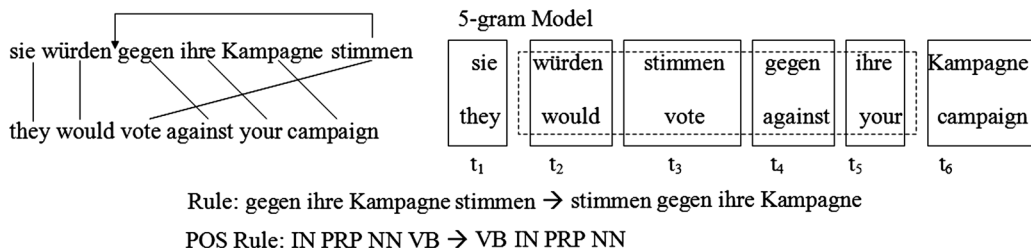
Figure 2 POS-based reordering in N-gram-based SMT: Learned rules.
